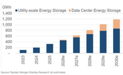
Exhibit 28: ...including utility-scale ESS in power markets
